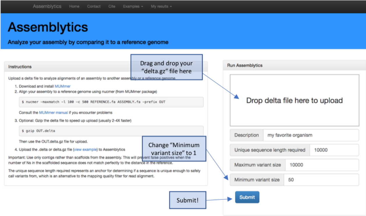
Figure 6. Assemblytics homepage and upload instructions
